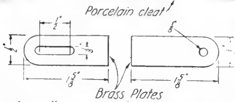
An easily constructed anchor-gap which may also be used as a plain gap for an ordinary spark-coil
